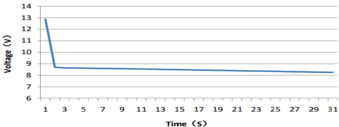
Cold Cranking Test Graph (-18°C, 450CCA)
