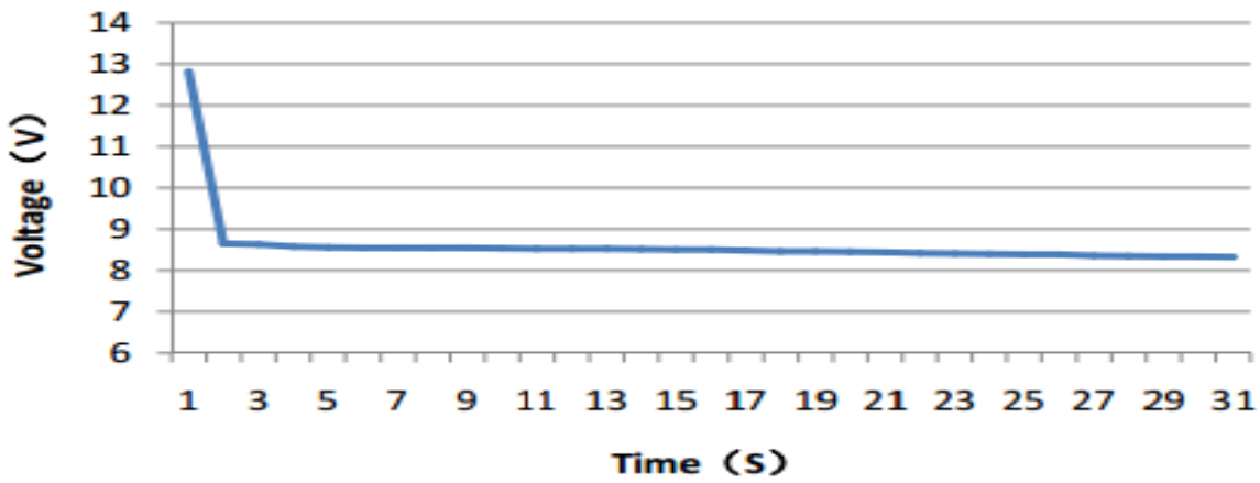
Cold Cranking Test Graph (-18°C, 700CCA)
