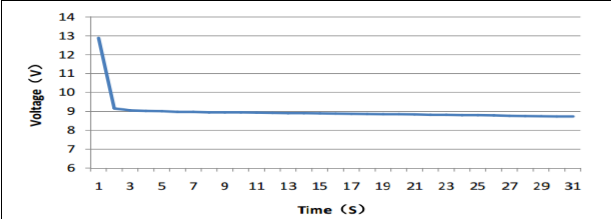
Cold Cranking Test Graph (-18°C, 1450CCA)
