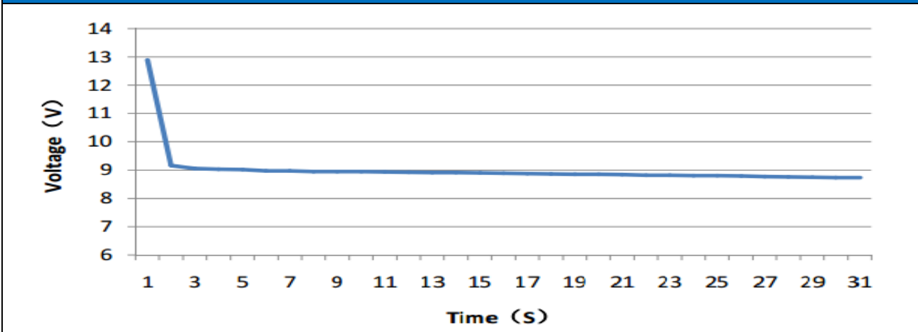
Cold Cranking Test Graph (-18°C, 1050CCA)
