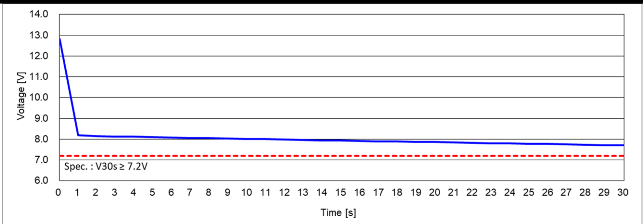
Cold Cranking Test Graph (-18°C, Icc 750A)
