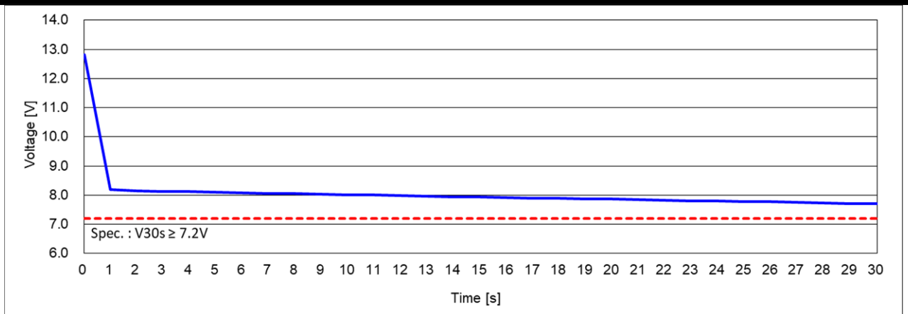
Cold Cranking Test Graph (-18°C, Icc 750A)
