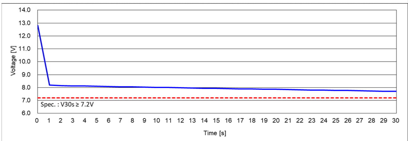
Cold Cranking Test Graph (-18°C, Icc 340A)
