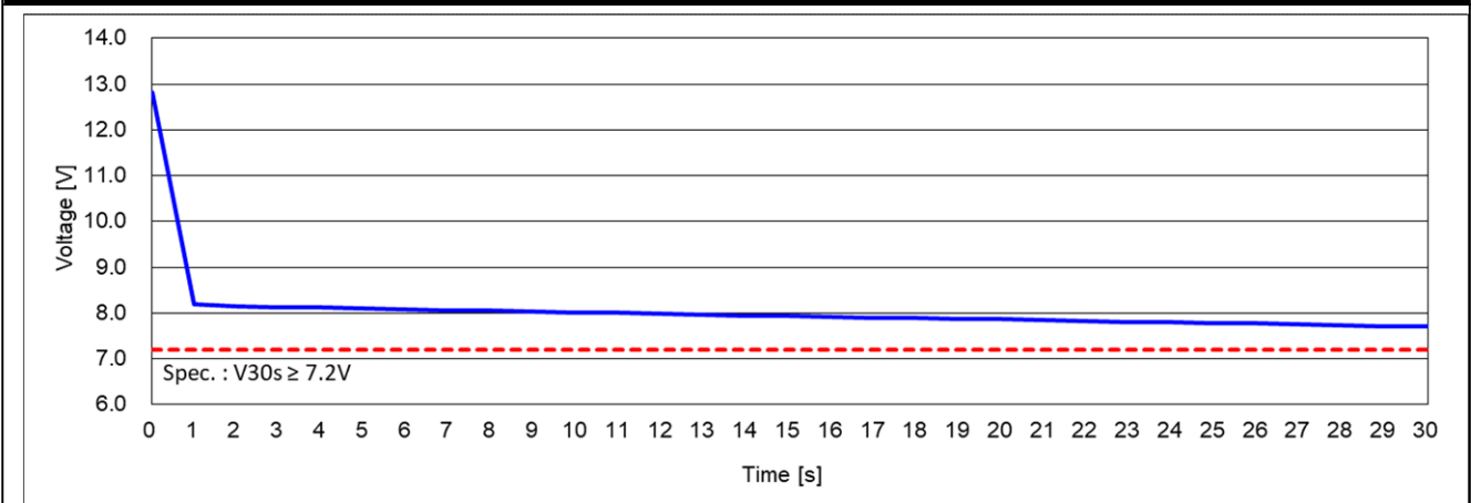
Cold Cranking Test Graph (-18°C, Icc 430A)
