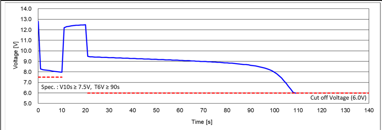
Cold Cranking Test Graph (-18°C, Icc 360A)
