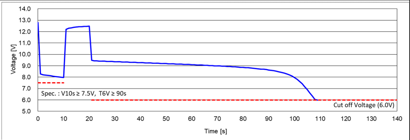
Cold Cranking Test Graph (-18°C, Icc 410A)
