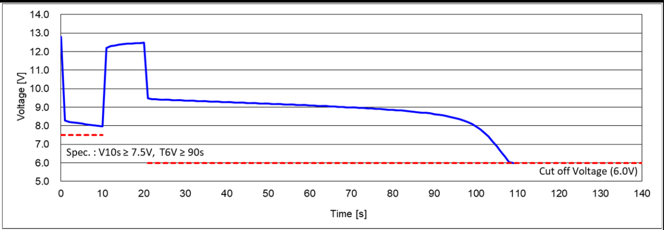
Cold Cranking Test Graph (-18°C, Icc 500A)
