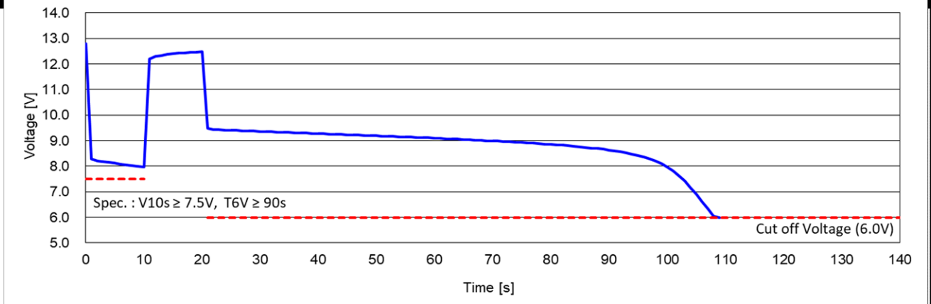
Cold Cranking Test Graph (-18°C. Icc 650A)
