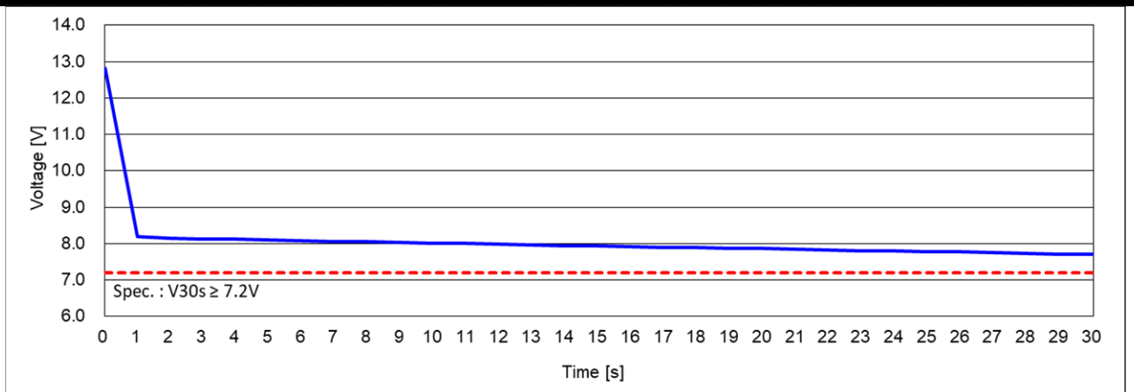
Cold Cranking Test Graph (-18°C, Icc 490A)
