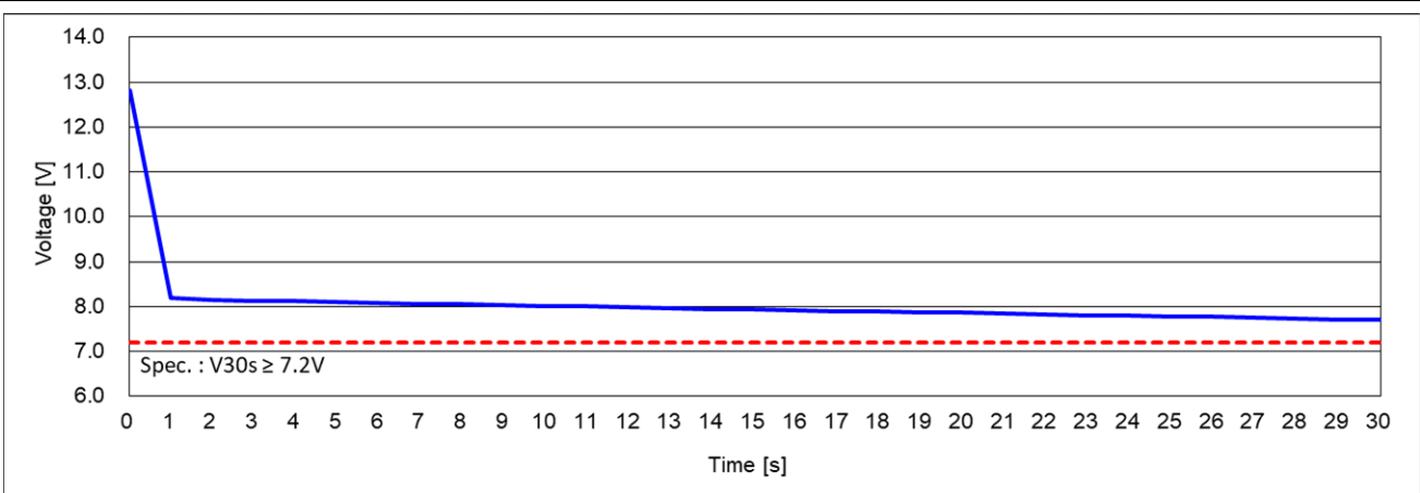
Cold Cranking Test Graph (-18°C, Icc 550A)
