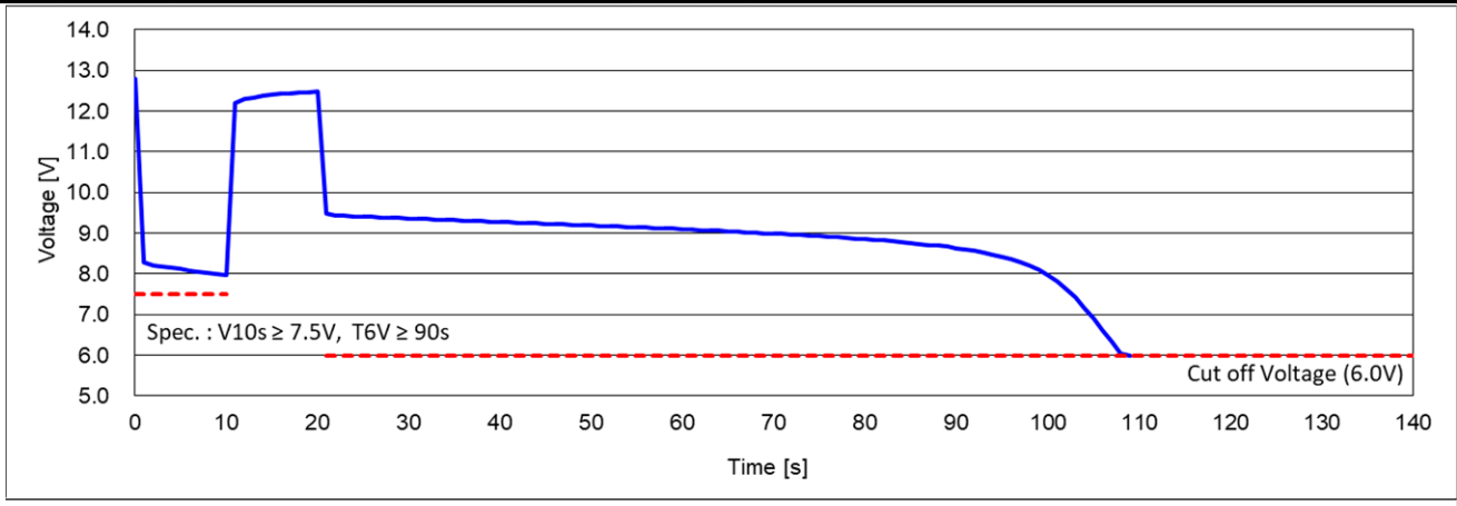
Cold Cranking Test Graph (-18°C, Icc 700A)
