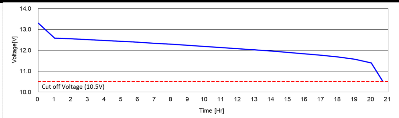
20HR Capacity Test Graph
