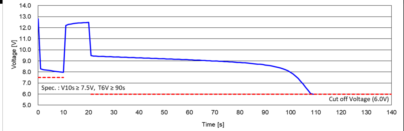
Cold Cranking Test Graph (-18°C. Icc 700A)
