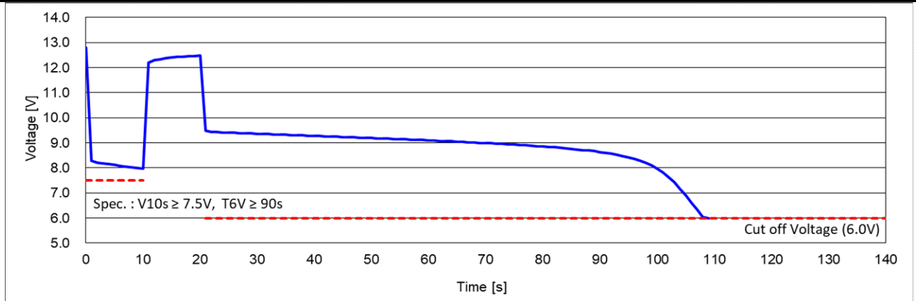
Cold Cranking Test Graph (-18°C, Icc 830A)
