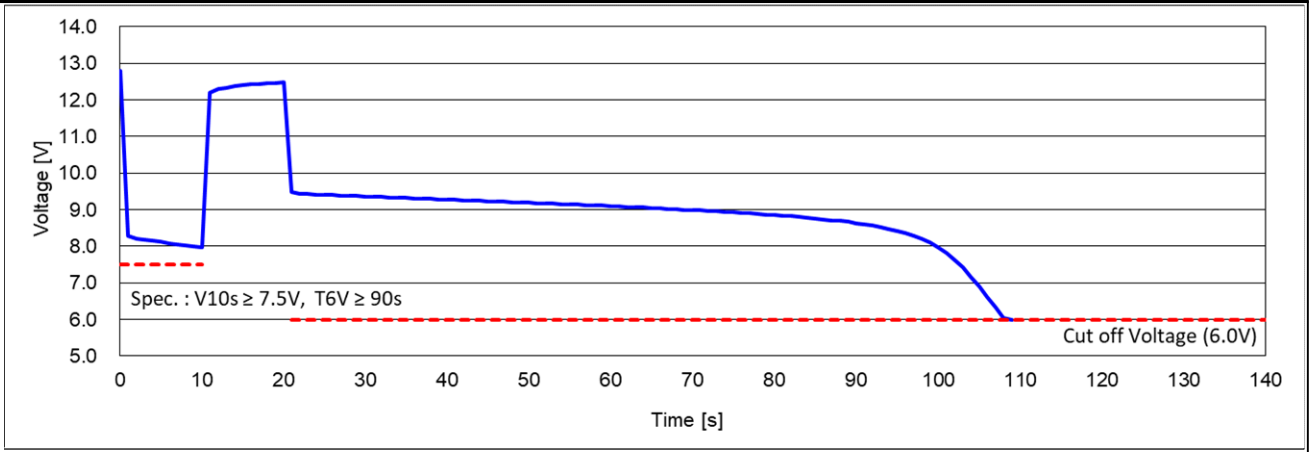
Cold Cranking Test Graph (-18°C, Icc 820A)
