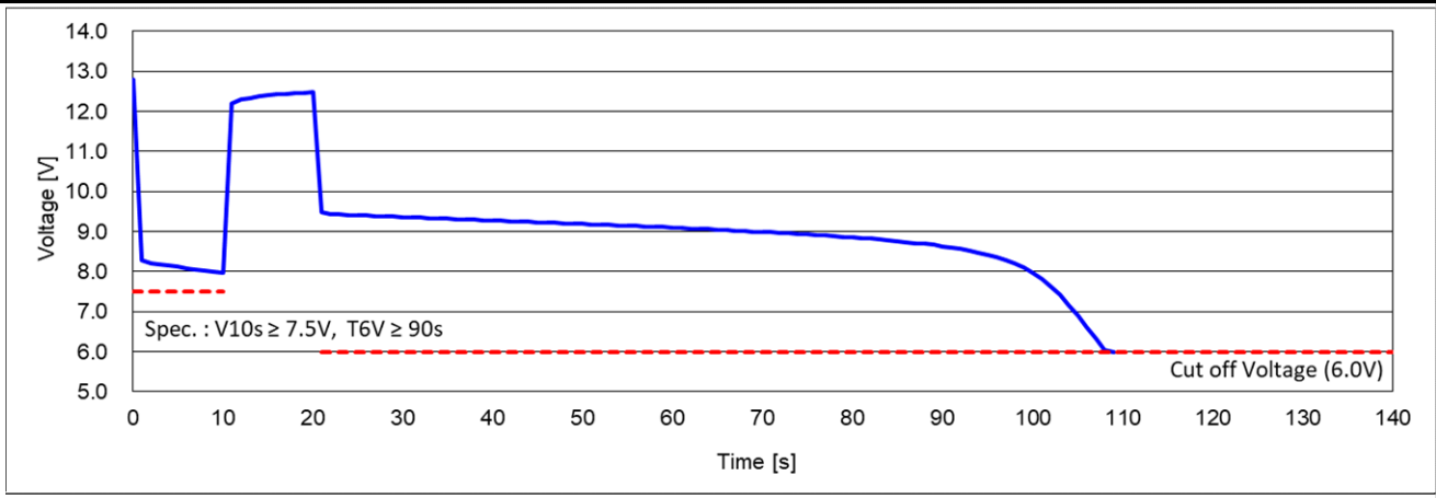
Cold Cranking Test Graph (-18°C, Icc 780A)
