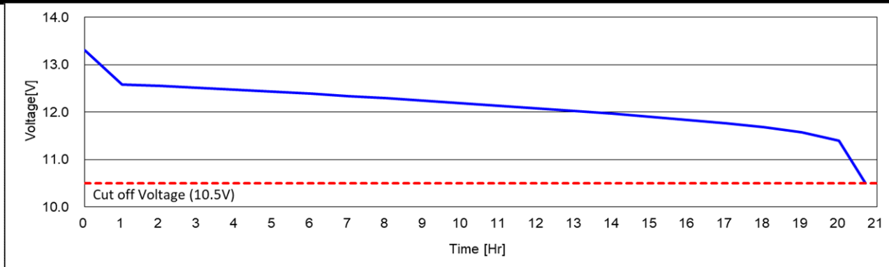
20HR Capacity Test Graph
