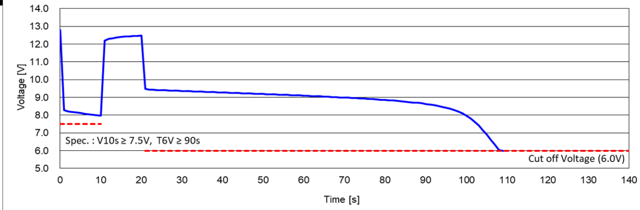
Cold Cranking Test Graph (-18°C. Icc 820A)
