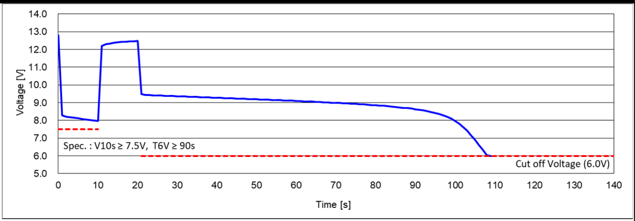
Cold Cranking Test Graph (-18°C, Icc 750A)
