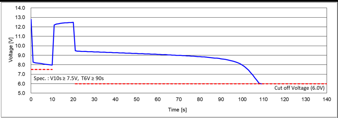
Cold Cranking Test Graph (-18°C, Icc 950A)
