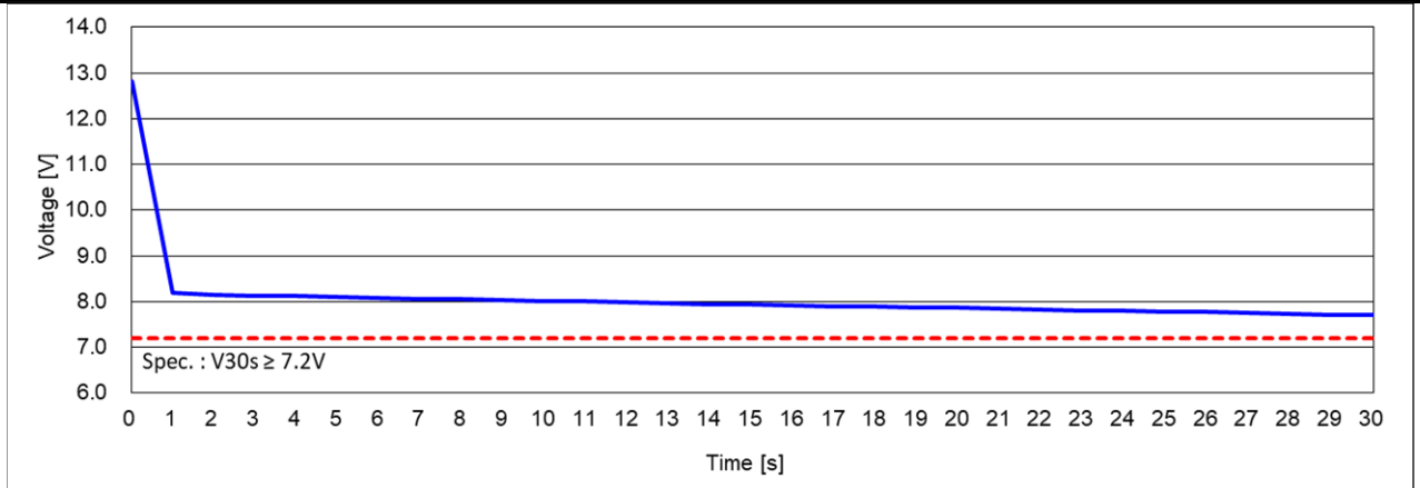
Cold Cranking Test Graph (-18°C, Icc 670A)
