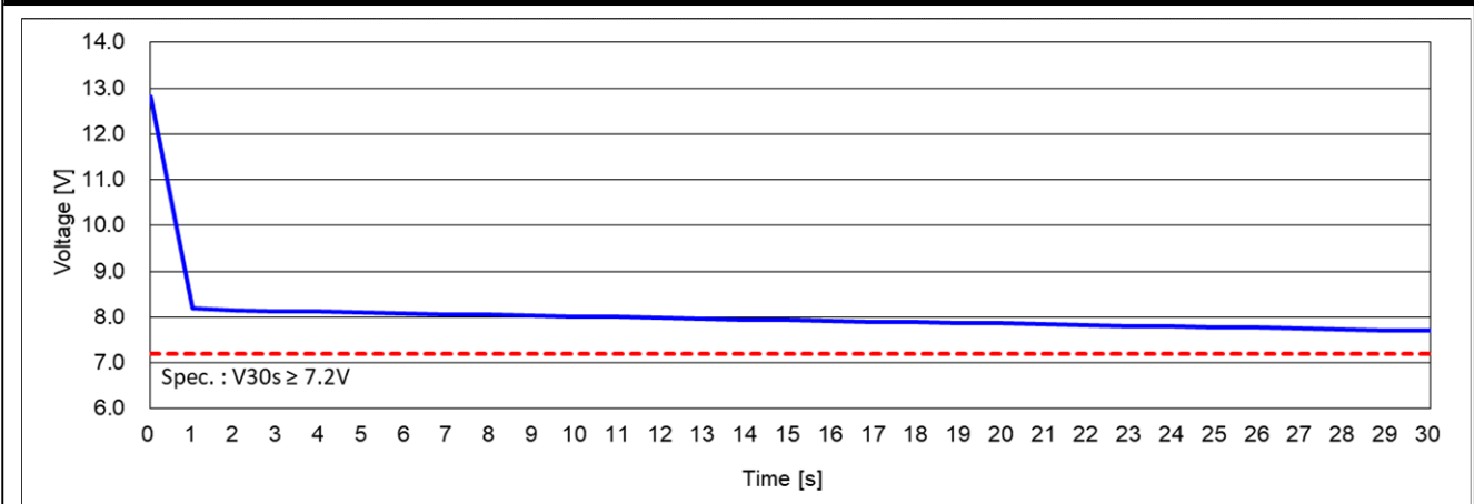
Cold Cranking Test Graph (-18°C, Icc 750A)
