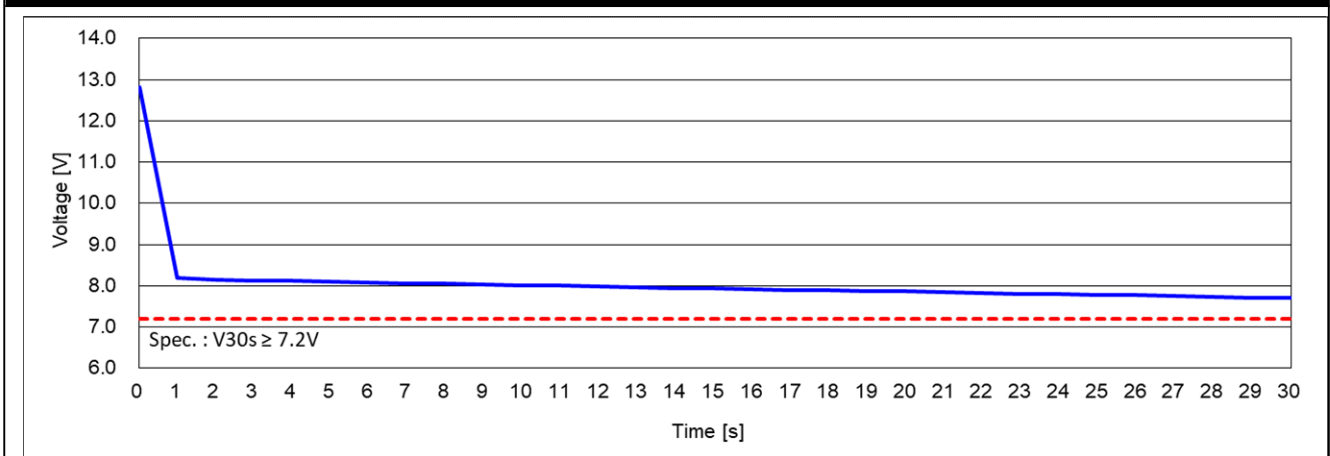
Cold Cranking Test Graph (-18°C, Icc 600A)
