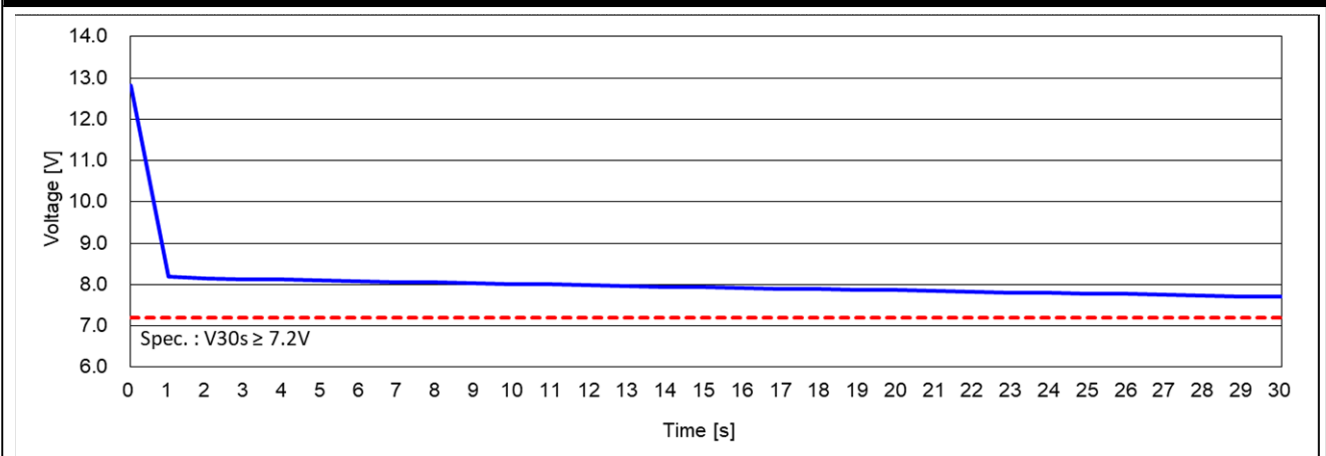
Cold Cranking Test Graph (-18°C, Icc 550A)
