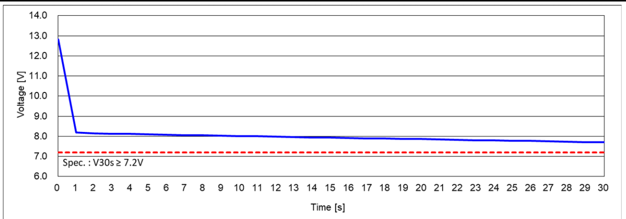
Cold Cranking Test Graph (-18°C, Icc 450A)
