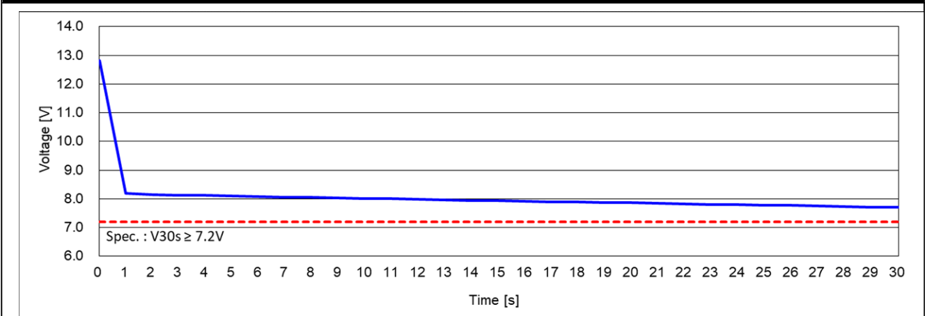
Cold Cranking Test Graph (-18°C, Icc 620A)
