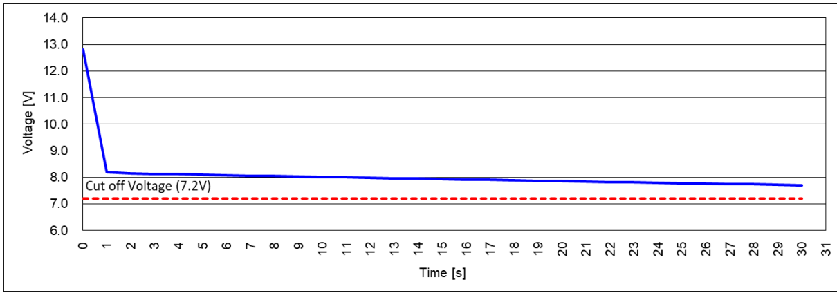
Cold Cranking Test Graph (-18 °C, Icc 900A)
