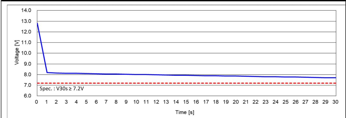
Cold Cranking Test Graph (-18°C, Icc A)
