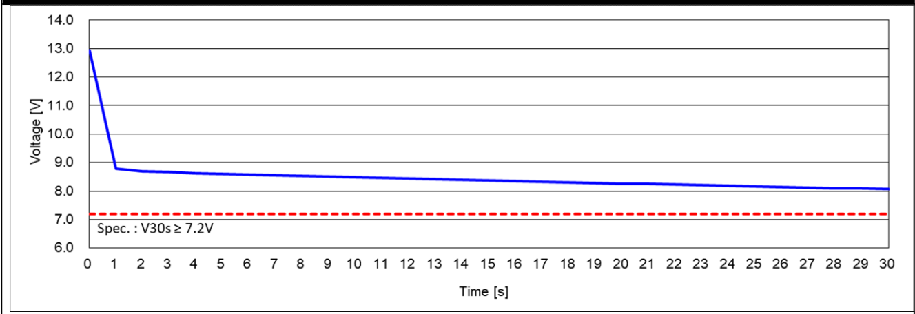
Cold Cranking Test Graph (-18°C, Icc 670A)
