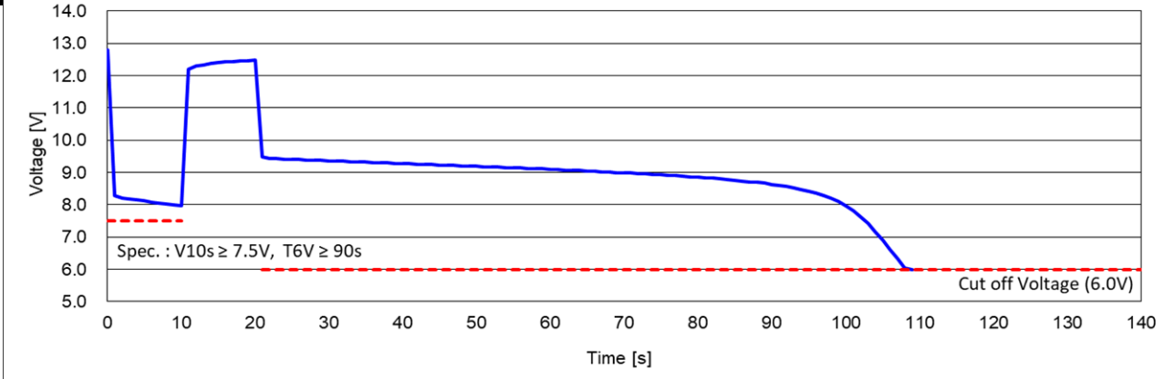
Cold Cranking Test Graph (-18°C. Icc 670A)
