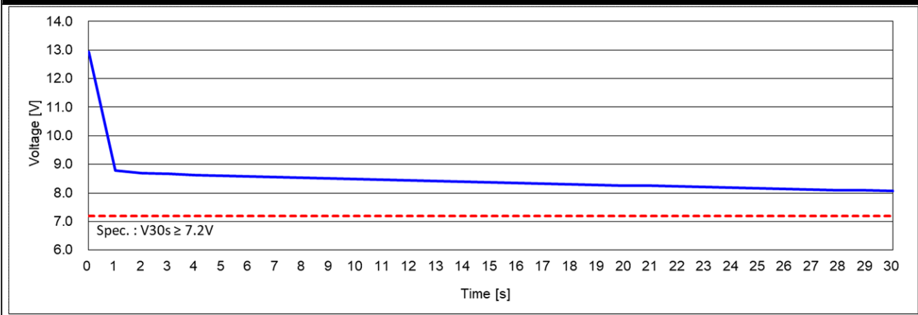
Cold Cranking Test Graph (-18°C, Icc 700A)
