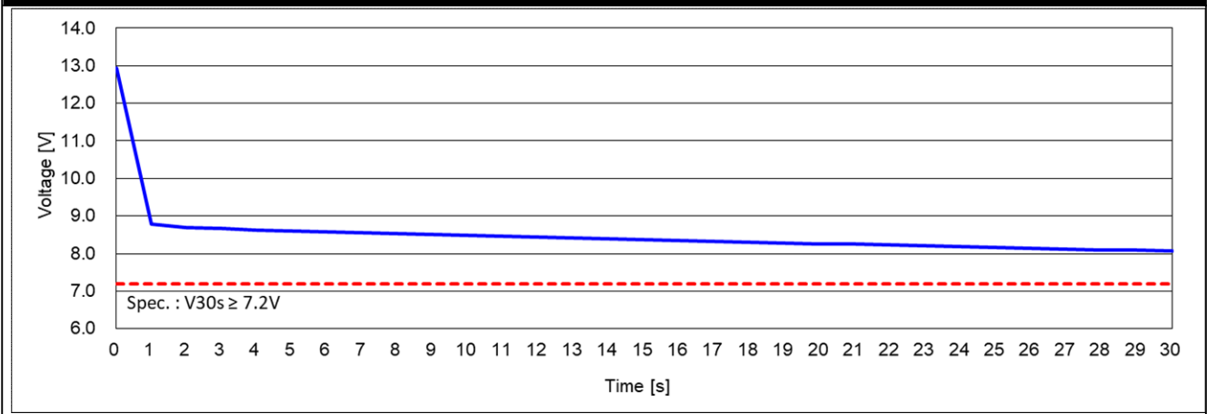
Cold Cranking Test Graph (-18°C, Icc 780A)
