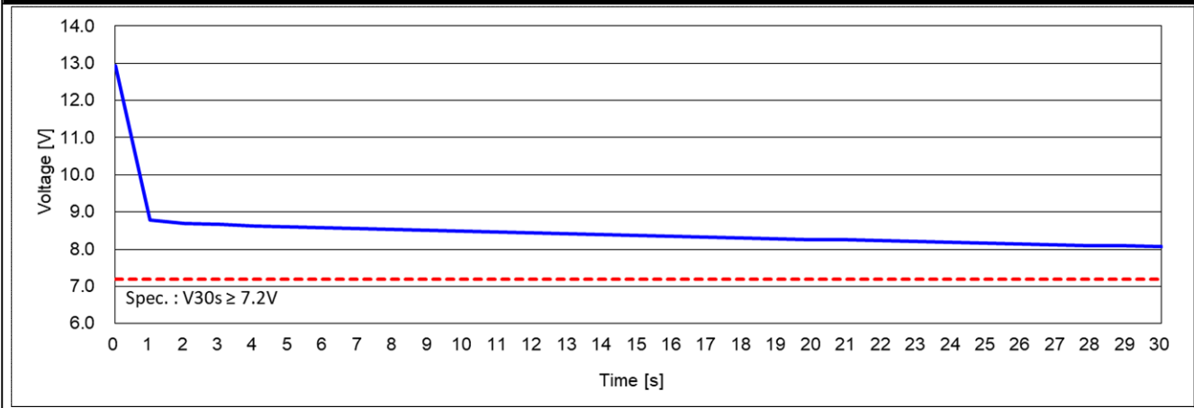
Cold Cranking Test Graph (-18°C, Icc 950A)
