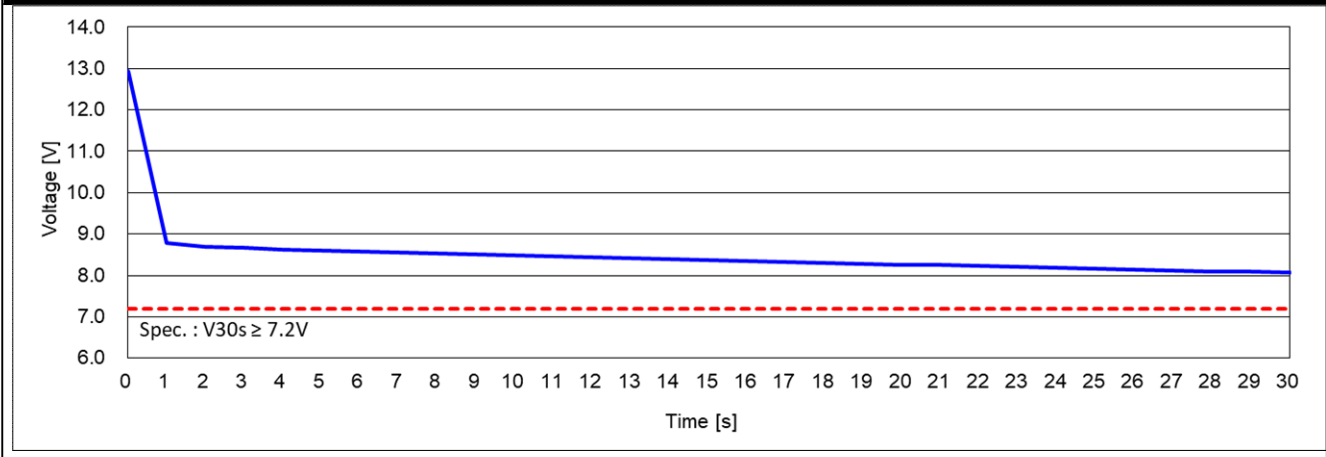
Cold Cranking Test Graph (-18°C, Icc 800A)
