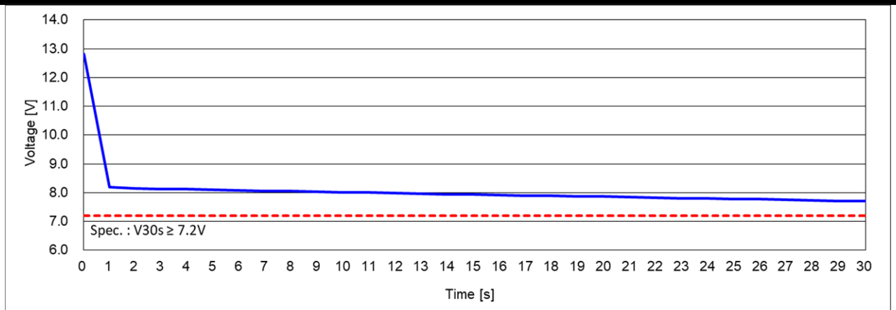
Cold Cranking Test Graph (-18°C, Icc 1000A)
