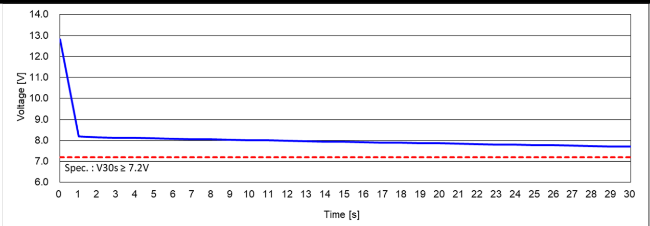
Cold Cranking Test Graph (-18°C, Icc 1000A)
