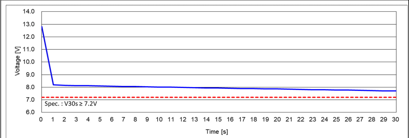
Cold Cranking Test Graph (-18°C, Icc 650A)
