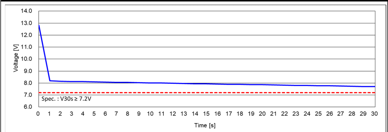
Cold Cranking Test Graph (-18°C, Icc 900A)
