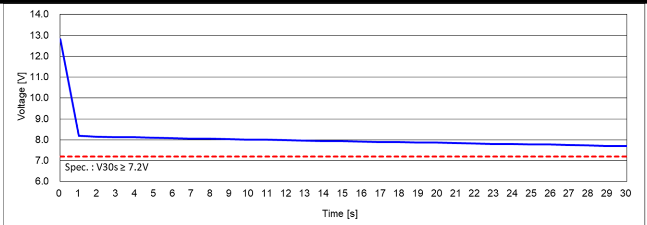
Cold Cranking Test Graph (-18°C, Icc 830A)
