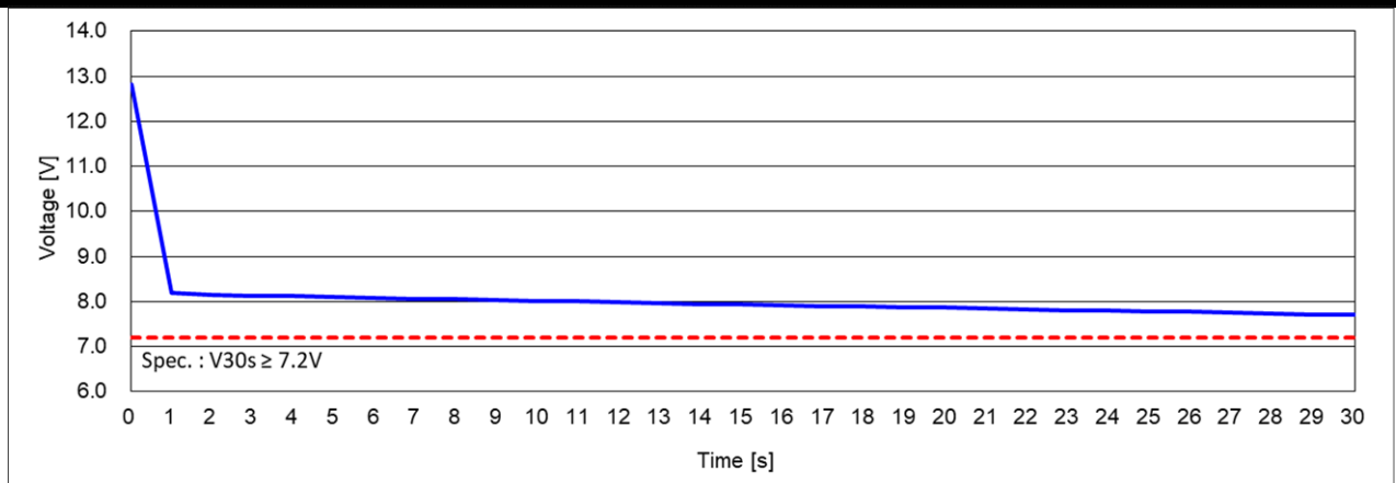
Cold Cranking Test Graph (-18°C, Icc 830A)
