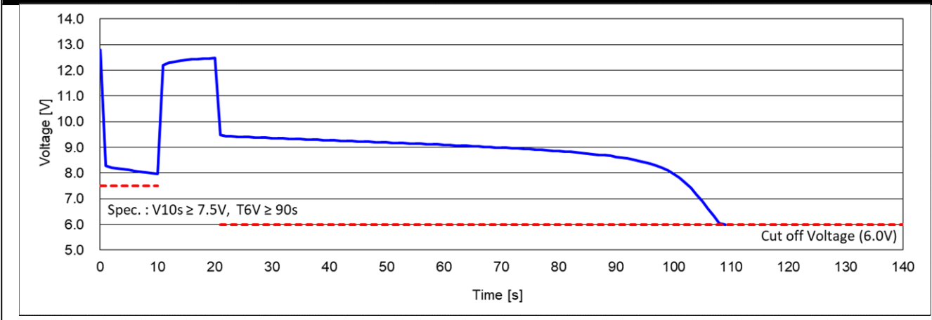
Cold Cranking Test Graph (-18°C, Icc 1000A)
