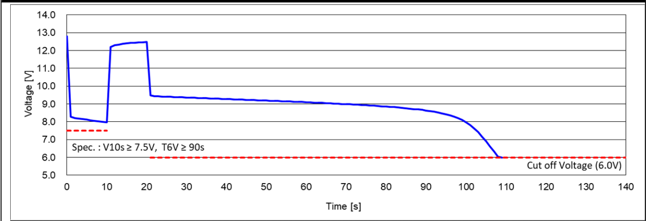
Cold Cranking Test Graph (-18°C, Icc 1250A)
