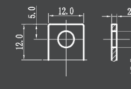
B1/B1B Terminal
