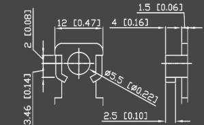
B3 Terminal
