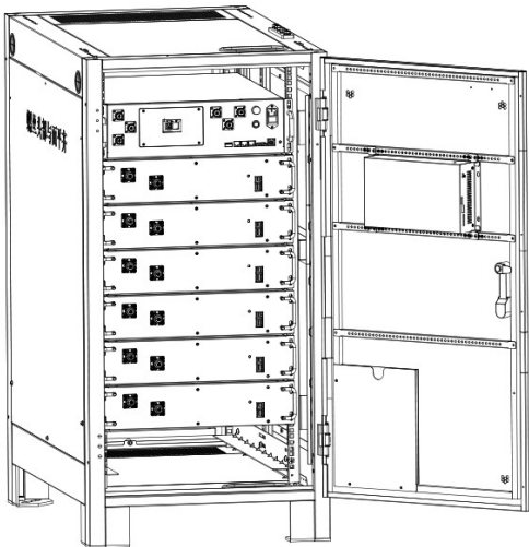
Rack 307.2V60Ah
