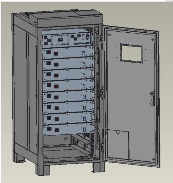
Rack 409.6V60Ah
