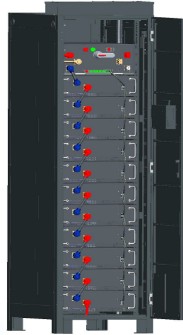
Rack TP220(S)
