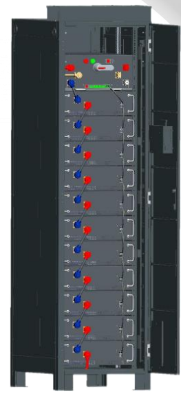
Rack TP220(S)
