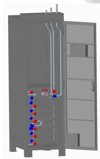
Rack TPH120(S)
